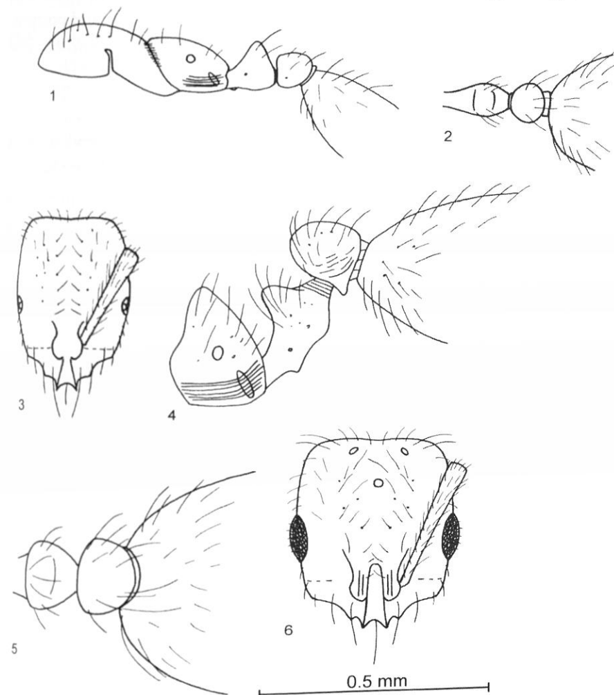
Figs 1-6. Solenopsis gnoma : 1, paratype worker, lateral view of mesosoma, petiole, postpetiole, and anterior part of gaster; 2, paratype worker, petiole and postpetiole as seen from above; 3, paratype worker, frontal view of head; 4, holotype female, lateral view of petiole, postpetiole, and anterior part of gaster; 5, holotype female, petiole and postpetiole as seen from above; 6, holotype female, frontal view of head. All figures are drawn to same scale.
