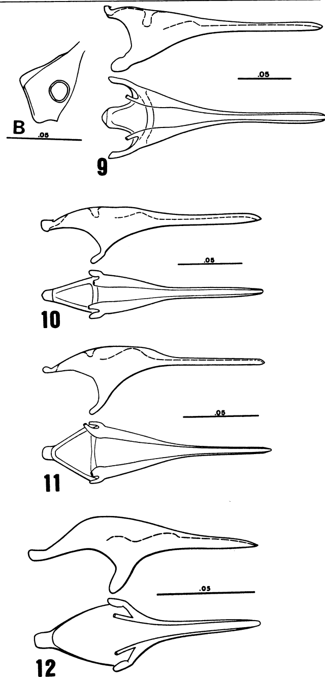
Figs. 8-12. Oligomyrmex . 8. O. corniger . A. Spiracular and quadrate plate of major worker. B. Spiracular plate of minor worker. 9. O. corniger major worker sting and furcula in lateral view (above) and ventral view (below). 10. O. corniger minor worker sting and furcula in lateral and ventral views. 11. O. overbecki major worker sting and furcula in lateral and ventral views. 12. O. urichi minor worker sting and furcula in lateral and ventral views.
