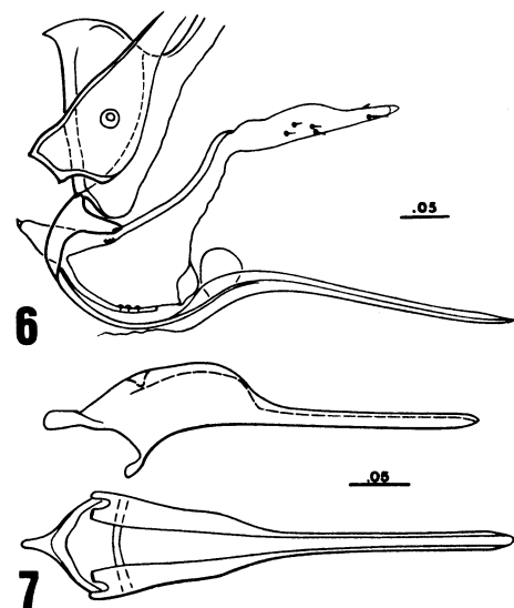
Figs. 6-7. Pheidologeton pygmaeus . 6. Right side of minor worker sting apparatus minus sting and furcula; gonostylus in ventral view. 7. Lateral view, sting and furcula of minor worker (above); ventral view, major worker (below).
