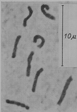
Abb. 15. Stenamma brevicorne . 2n = 8 . Neuroblastenmitose.
