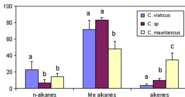
Fig. 6. PPG content of the main hydrocarbon classes for three Cataglyphis species (mean% \pm SD). Different letters indicate significant differences.
