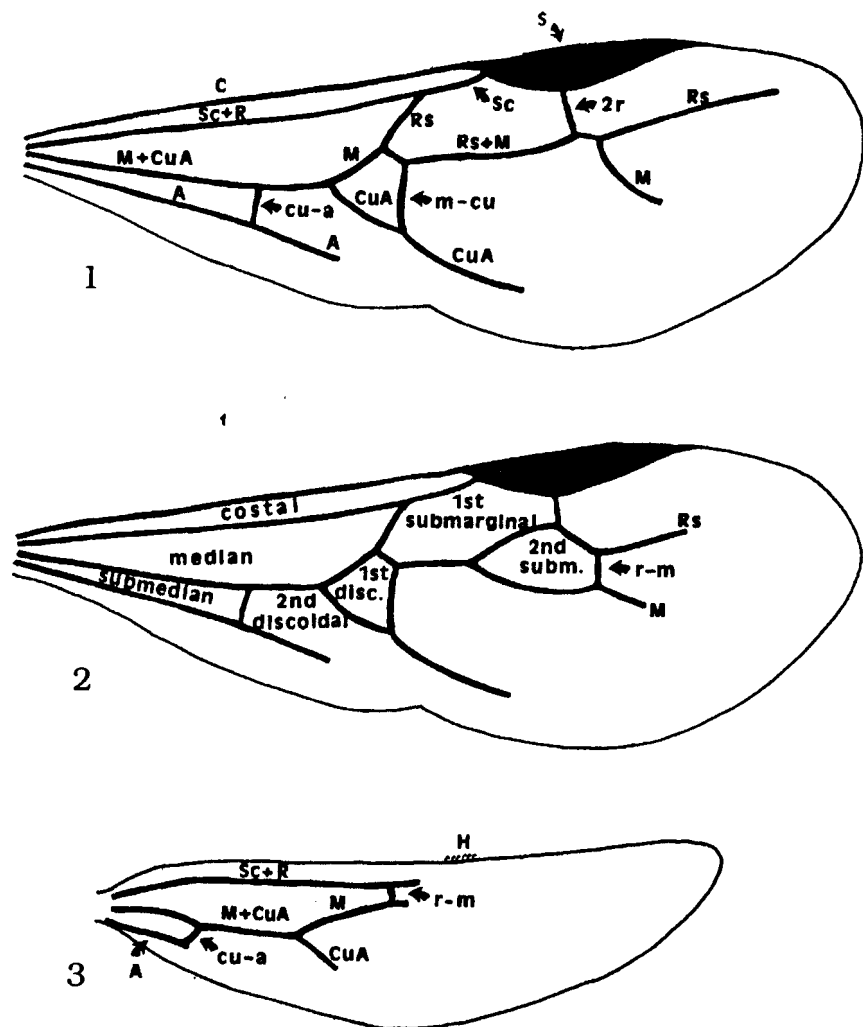
Figs. 1 - 3. Typical wing venation for Stenamamma species. 1. Veins of forewing. A — Anal, C — Costal, CuA — Cubito-Anal, cu-a — cubital to anal cross vein, M — Median, m-cu — medio-cubital cross vein, R — Radial, 2r — radial cross vein, RS — Radial sector, S - Stigma (pterostigma), Sc — Subcostal. 2. Cells of forewing. 1st disc. — 1st discoidal, 2nd subm. — 2nd submarginal. Veins as in Fig. 1. 3. Veins of hindwing. H — Hamuli. Veins as in Fig. 1. Magnification of these figures is variable.
